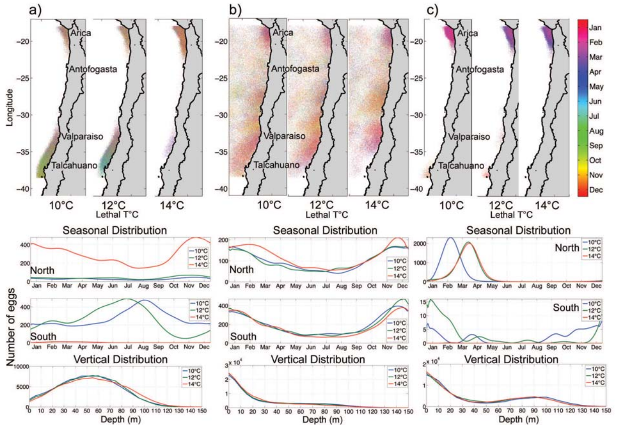
FIG. 4.4 – Emerging spawning patterns in the southern Humboldt Current system (off Chile) with different lethal temperatures (10°C, 12°C and 14°C) and different selective constraints: (a) shelf retention, (b) non-dispersion, (c) shelf retention and non-dispersion.
