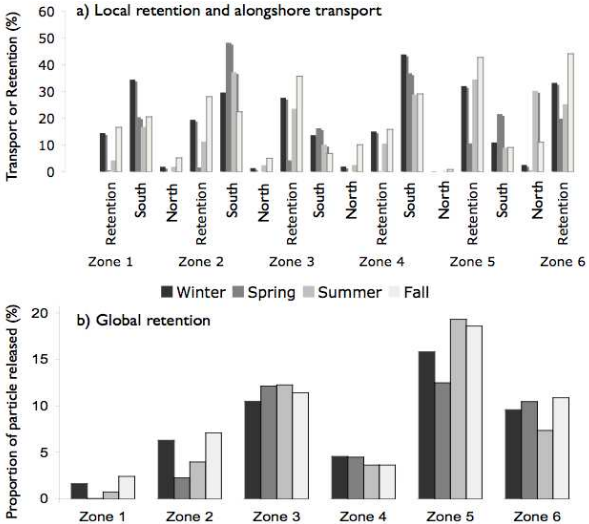
FIG. 3.4 – Alongshore transport (north or south) and retention for each release zone and for each season, Simulation I-A. (a) Local retention and alongshore transport. (b) Global retention of particles over the shelf.
