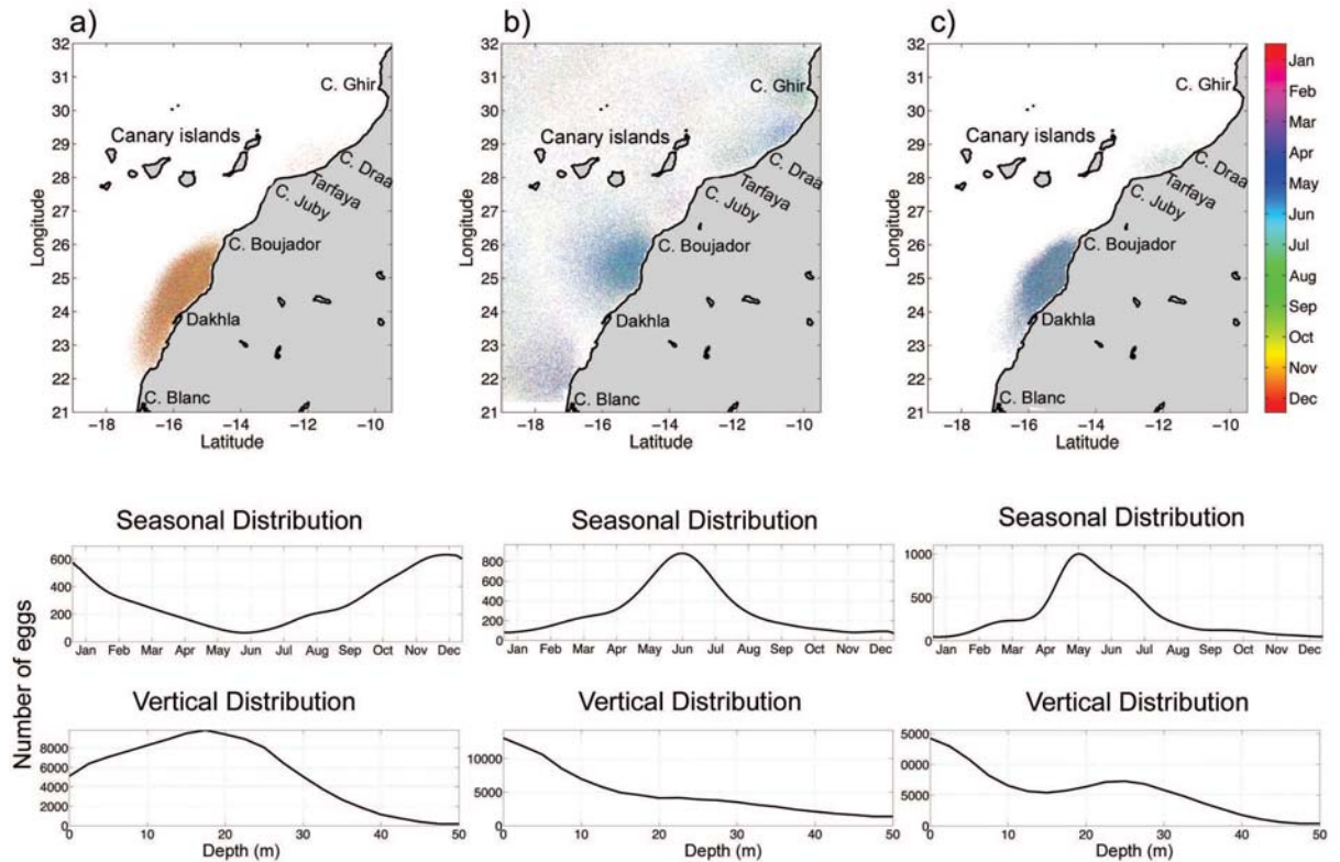
FIG. 4.2 – Emerging spawning patterns in the central Canary Current system (off Morocco) with a lethal temperature of 10^{\circ}\text{C} and different selective constraints: (a) shelf retention; (b) non-dispersion; (c) shelf retention and non-dispersion.
